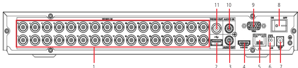
Painel traseiro
