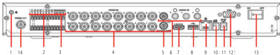
Painel traseiro
