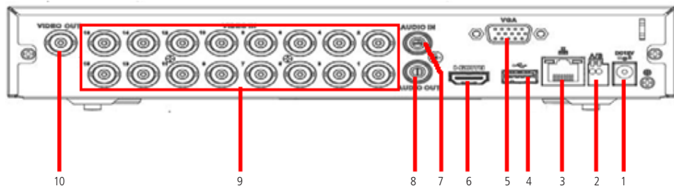
Painel traseiro
